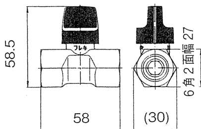
[FBS-100-15 型]
